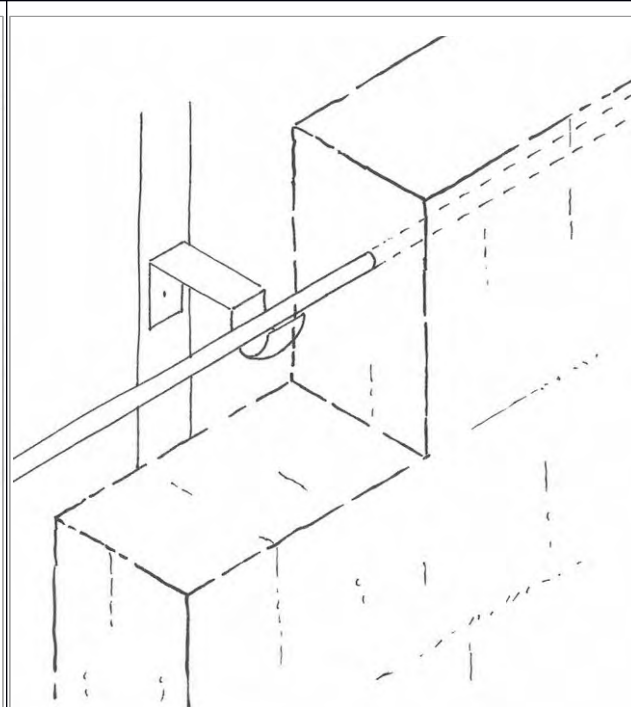
Figure 23: Liaison souple
