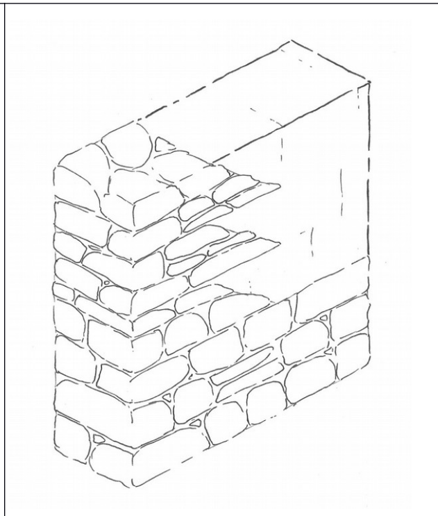
Figure 21: Jonction pierre/bauge
