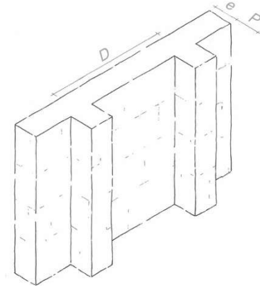
Figure 5: Contreforts*
