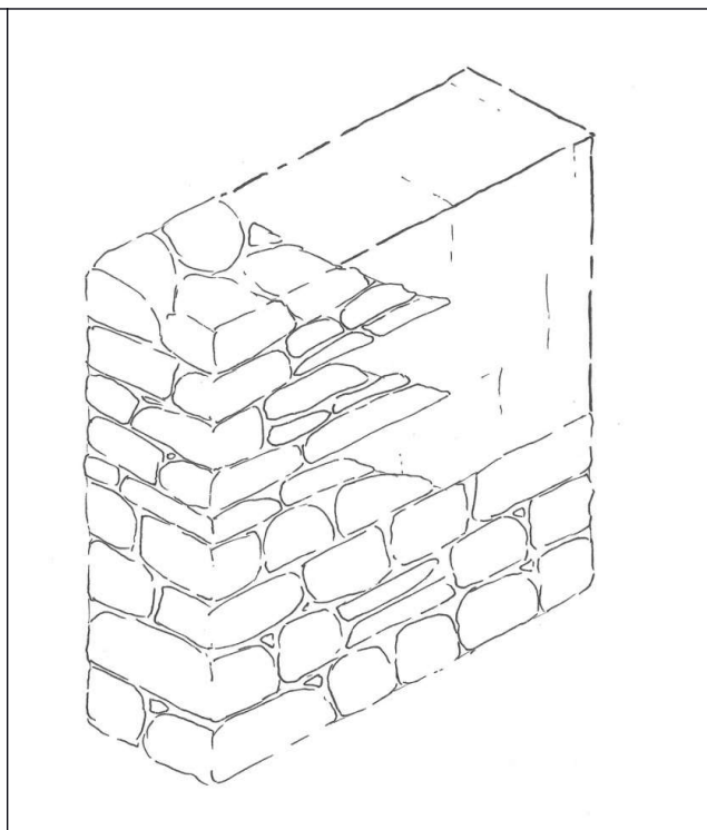
Figure 21: Jonction pierre/bauge
