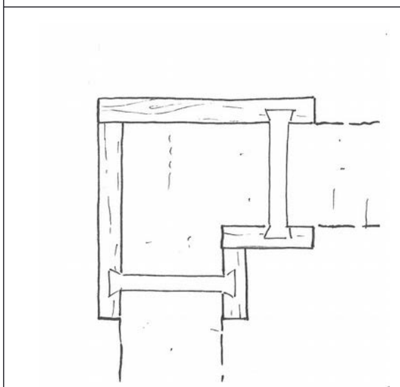
Figure 27: Agrafe* extérieure
