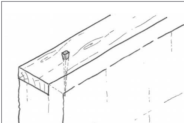
Figure 34: Simple sablière
