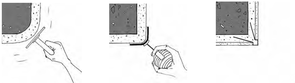
Figure 1: Protection des angles sortants
